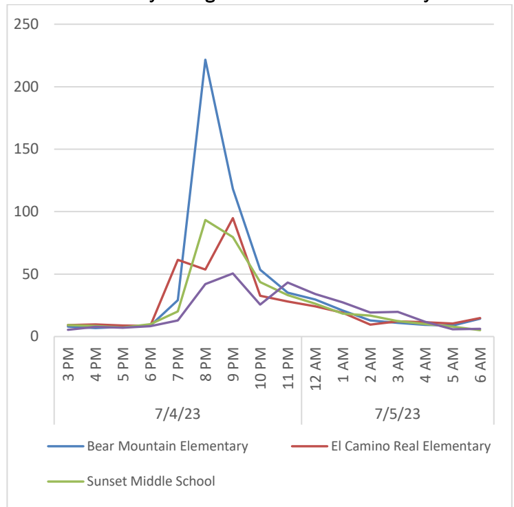
Hourly Average of PM2.5 on the 4 th of July
