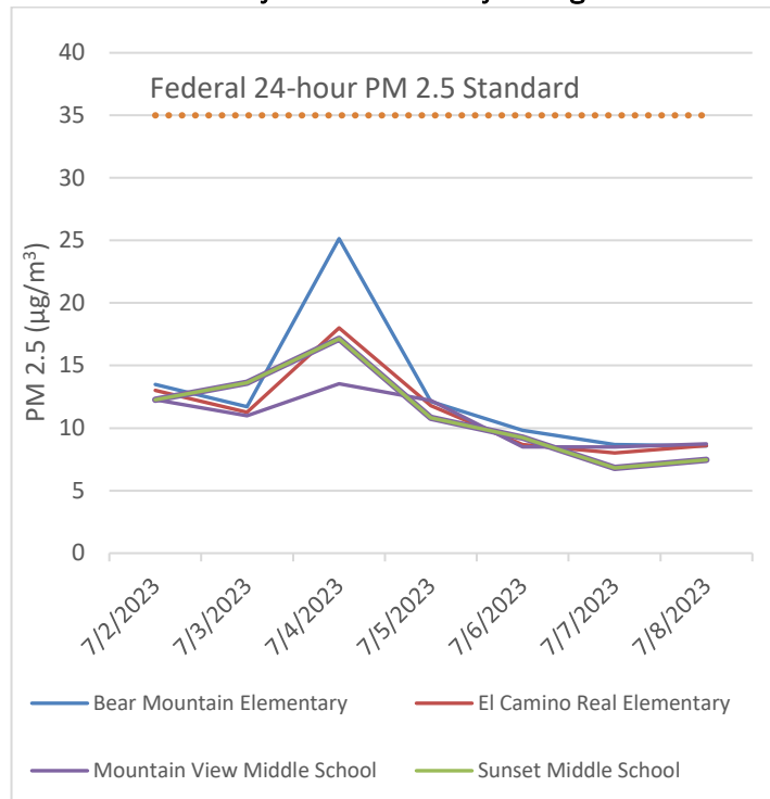
Weekly PM 2.5 24 Hourly Average
