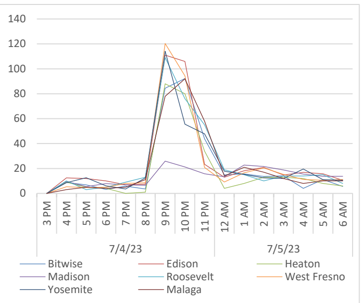
Hourly Average of PM2.5 on the 4th of July
