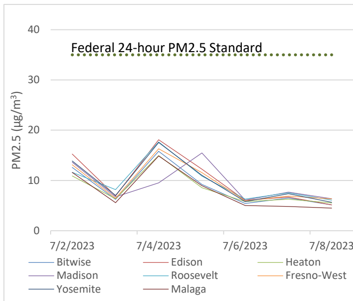
Weekly PM 2.5 24 Hourly Average
