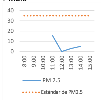
PM2.5
