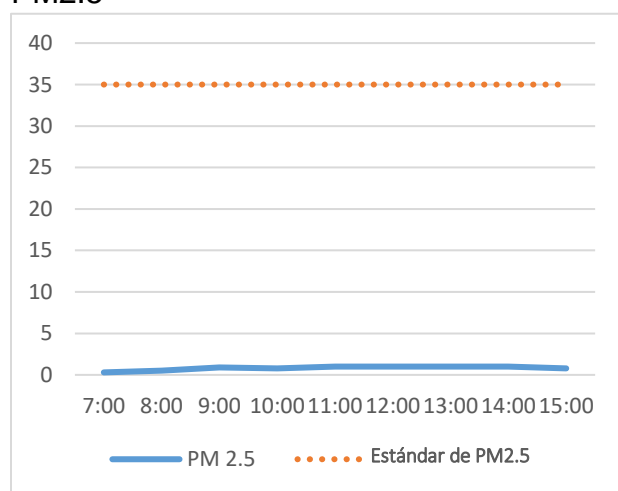
PM2.5
