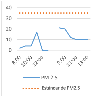
PM2.5
