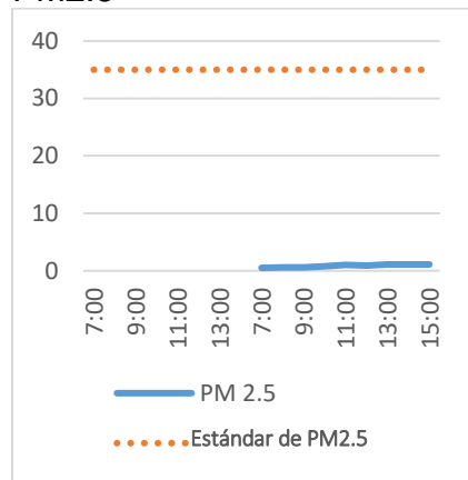
PM2.5
