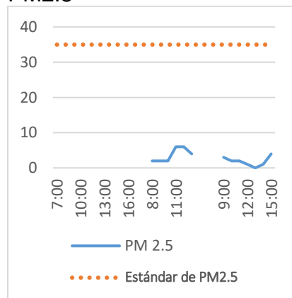
PM2.5
