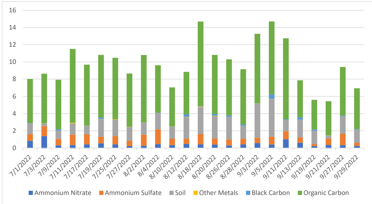
Figure 3 Speciated PM 2.5 Concentrations at Edison High School
