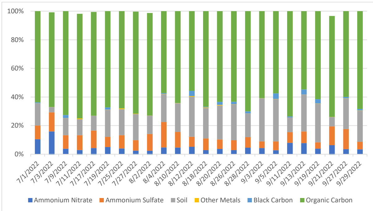
Figure 4 Relative Comparison of PM2.5 Species Measured at Edison High School
