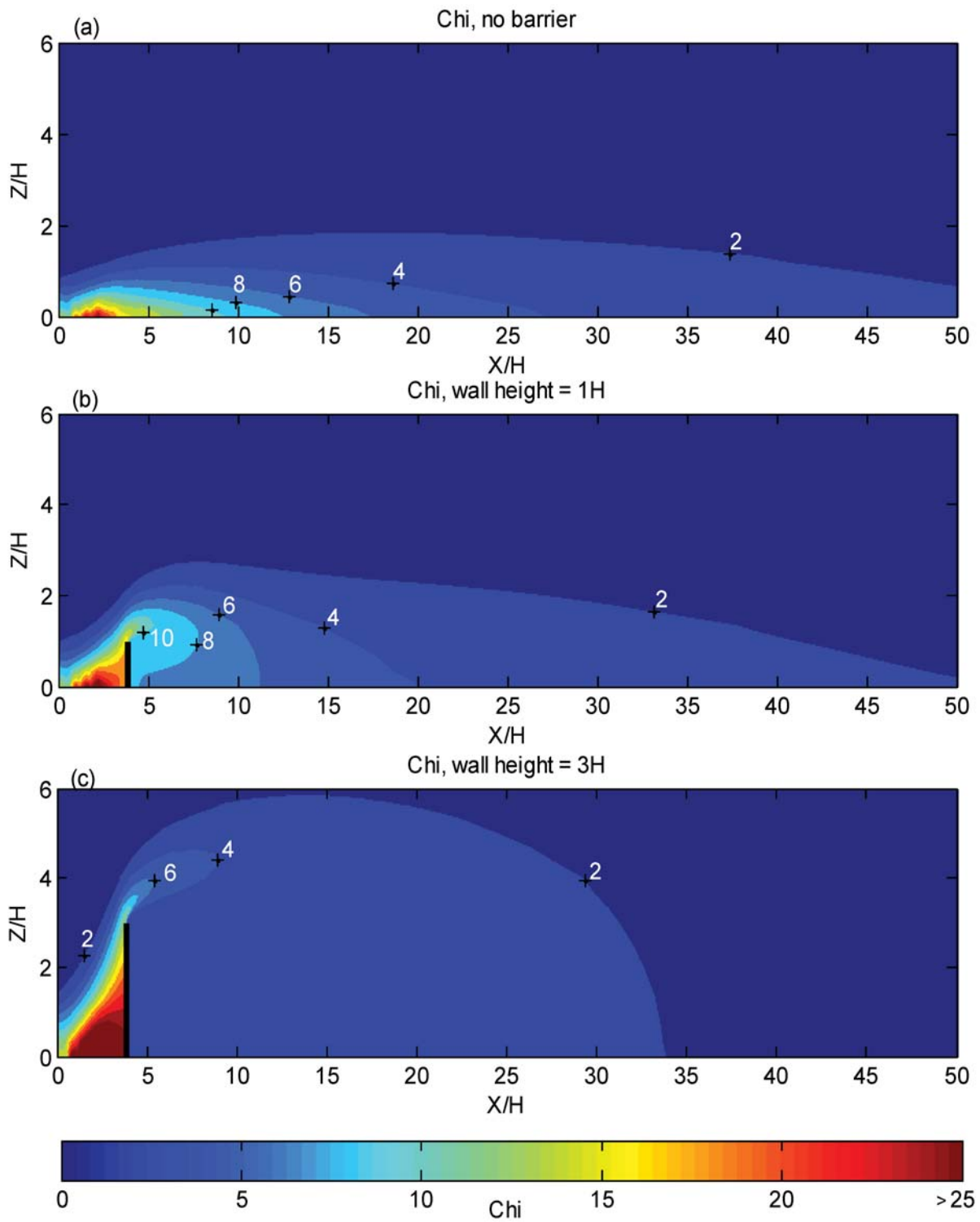
Figure 1. CFD modeling analysis of varying solid noise barrier heights. For the figure above, the top panel shows no barrier, the middle panel a barrier of height, H, and the bottom panel a barrier of height 3H. The distances downwind are also relative to the barrier height. As an example, for H=6 meters, the middle panel would represent a 6 meter tall barrier and the bottom panel an 18 meter tall barrier, and the x-axis distance values would also be multiplied by 6 meters. For this figure, Z represents the vertical height above ground and X the distance from the nearest travel lane on the road (Hagler et al, 2012).
