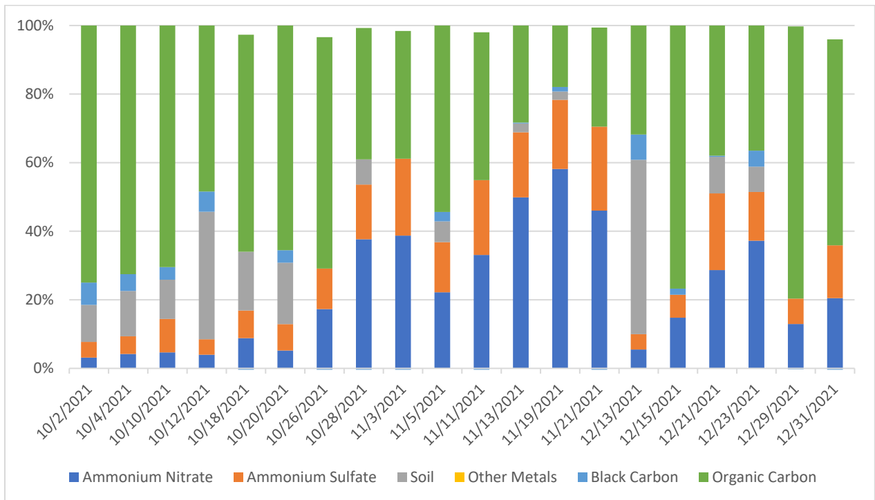
Figure 4 Relative Comparison of PM2.5 Species Measured at Shafter DMV Site
