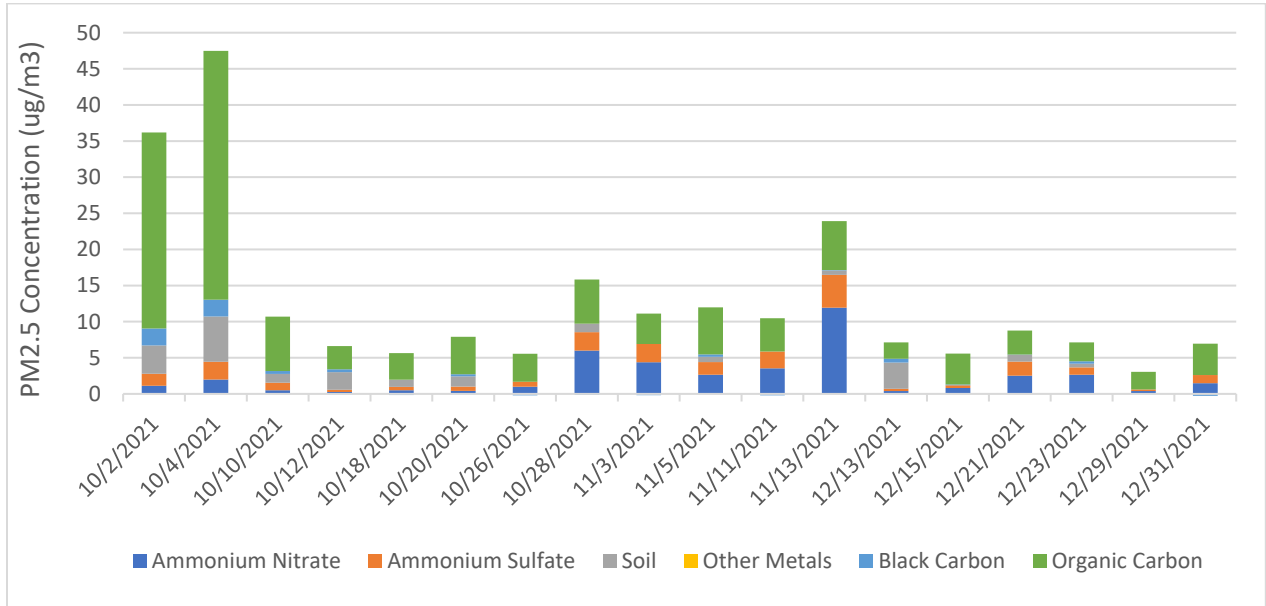
Figure 3 Speciated PM2.5 Concentrations at Shafter DMV Site
